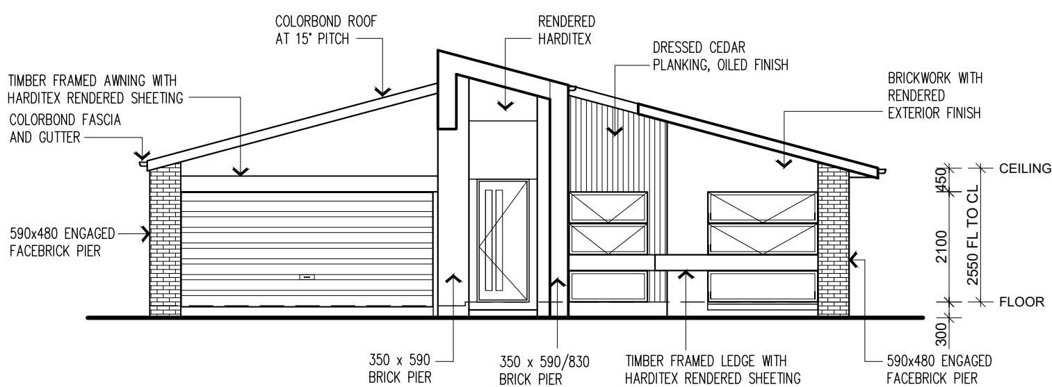
FRONT ELEVATION - ULTRA MODERN
